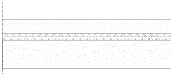
QuietMat WAVE 50 with 4" concrete topping
